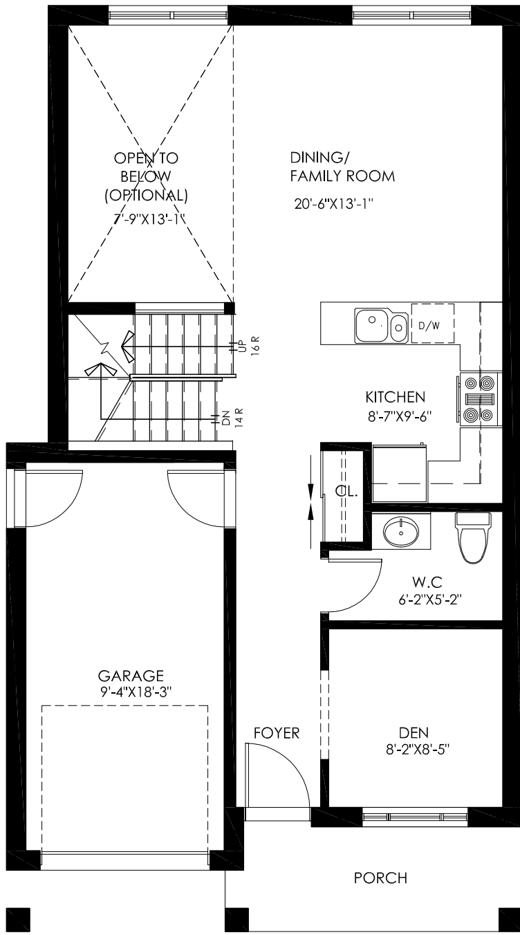
MAIN FLOOR PLAN: 720 SQ.FT.
