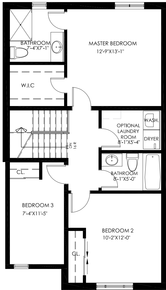
SECOND FLOOR PLAN: 805 SQ. FT.
