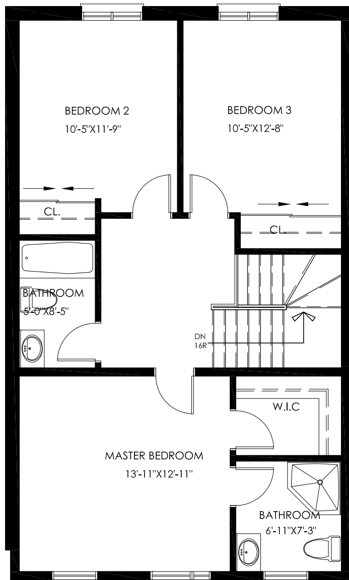
SECOND FLOOR PLAN: 830 SQ. FT.
