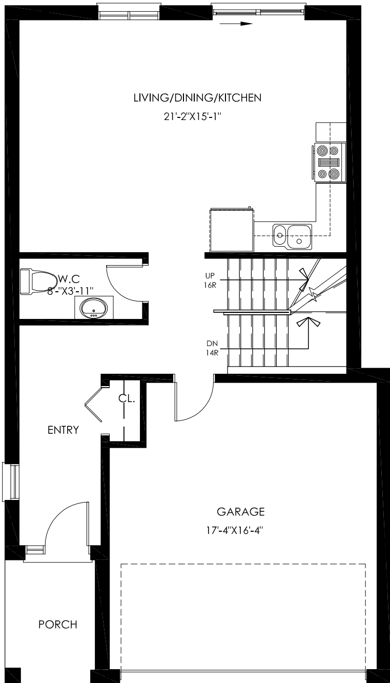
MAIN FLOOR PLAN: 651 SQ. FT.
