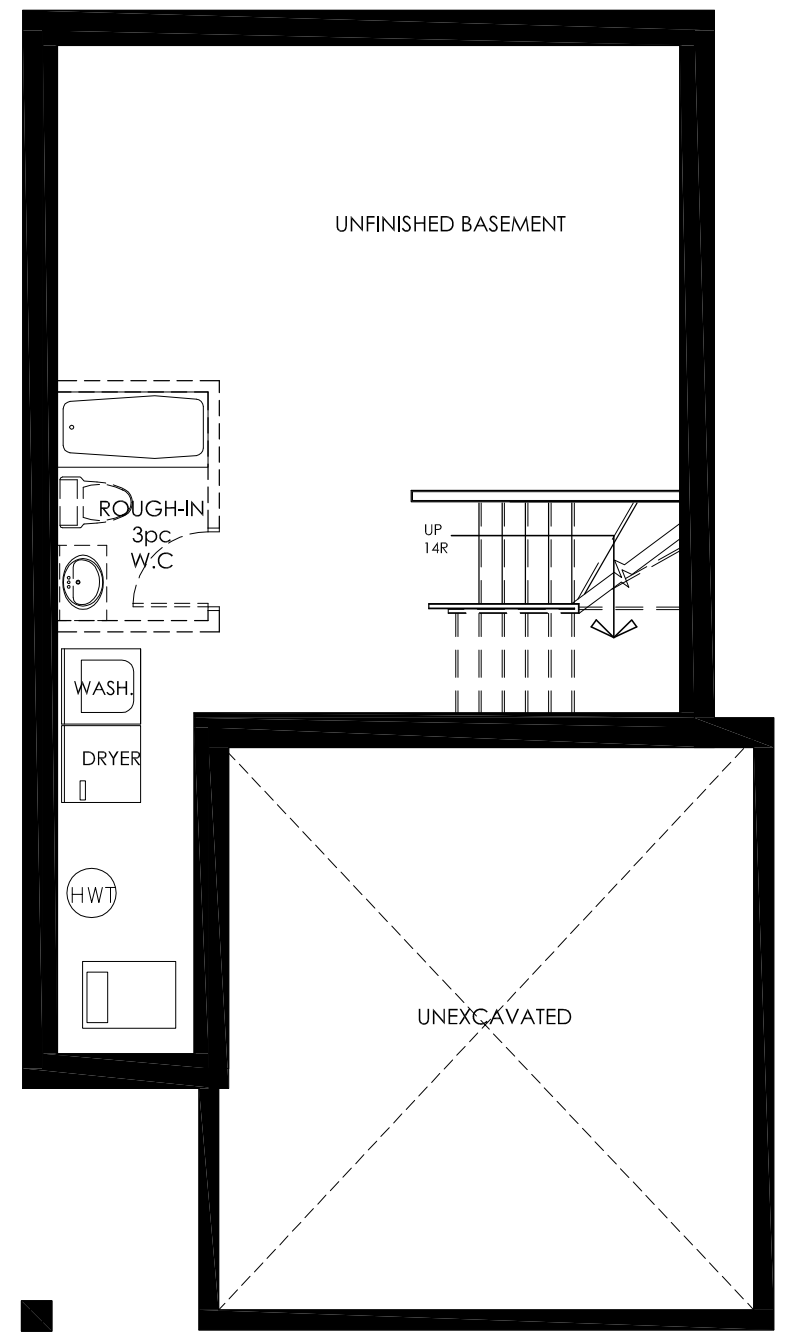
BASEMENT PLAN: 640 SQ. FT.
