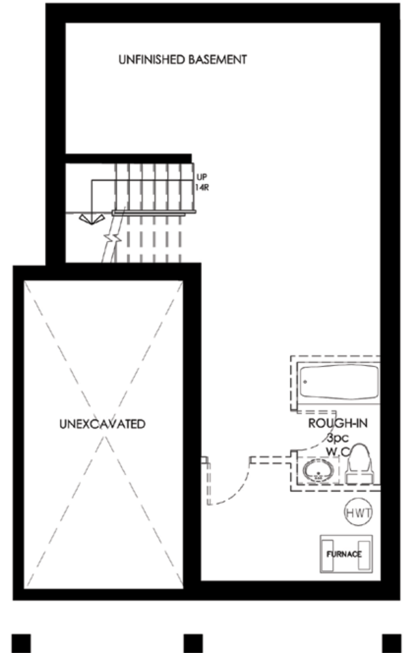
BASEMENT PLAN: 608SQ. FT.
