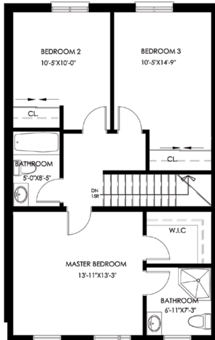
SECOND FLOOR PLAN: 788 SQ. FT.
