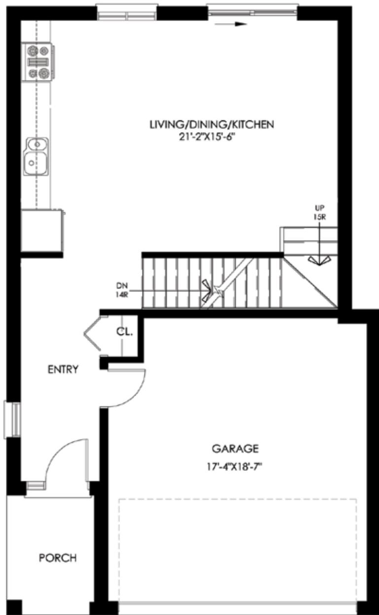
MAIN FLOOR PLAN: 567 SQ. FT.
